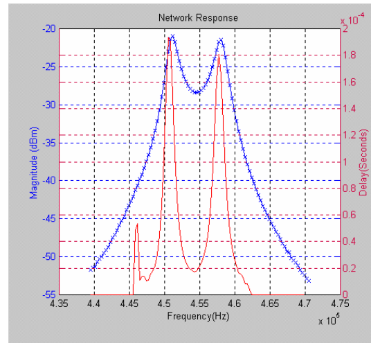
Figure 4 – 455 kHz Bandpass Filter
