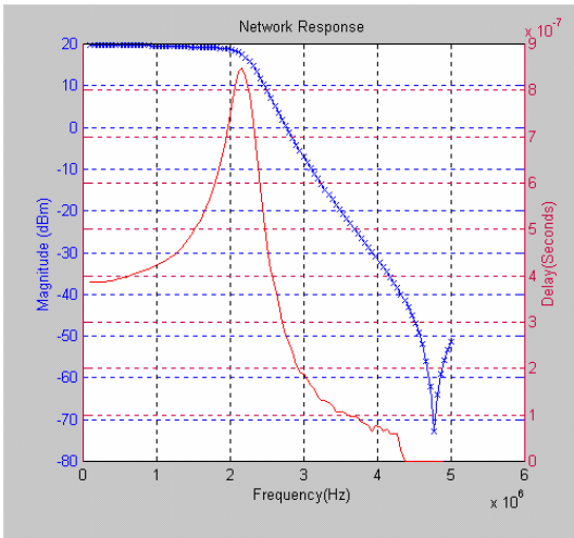
Figure 2 – 1.9 MHz Low Pass Filter
