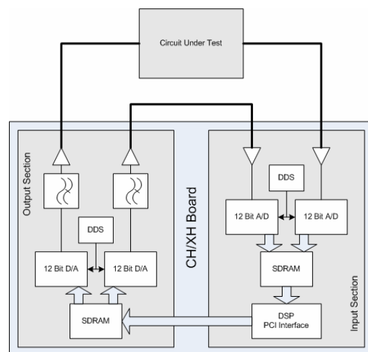
Figure 1 – CH/XH Block Diagram
